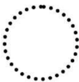
Ideal Circle
