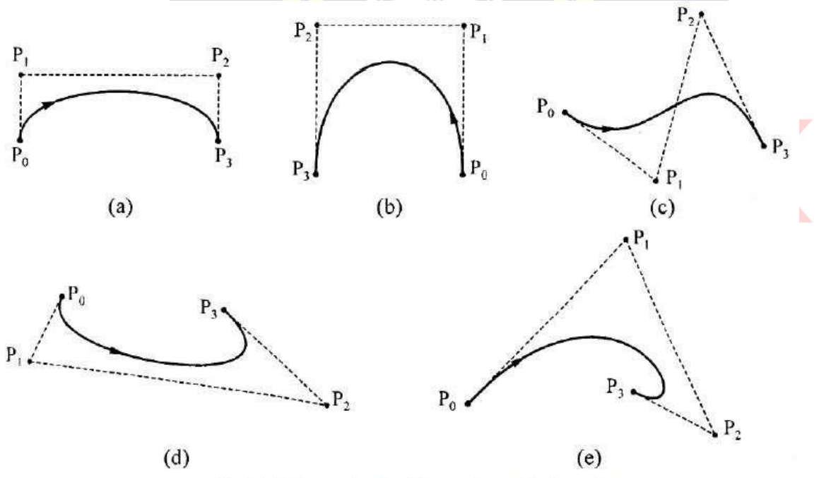
Fig. 2.17 Same Typical Examples of Beizer Curve
